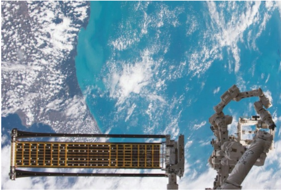
Our ROSA solar array was demonstrated on the International Space Station in 2017. Credit: NASA
