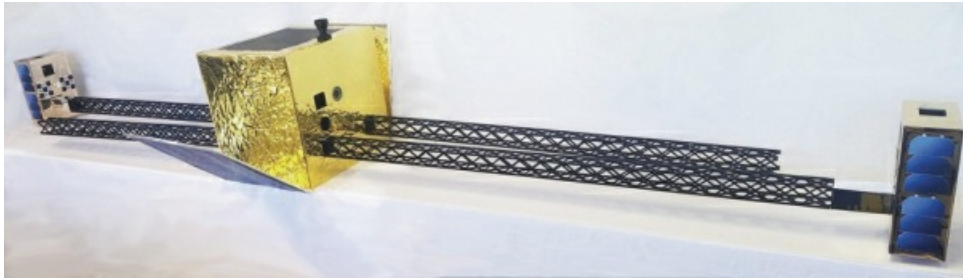
Optimast-SCI, a space assembled interferometer. Using on-orbit assembly and manufacturing, the system will deploy booms up to 50 m long that will allow high angular resolution observations to be made. Credit: Redwire.
